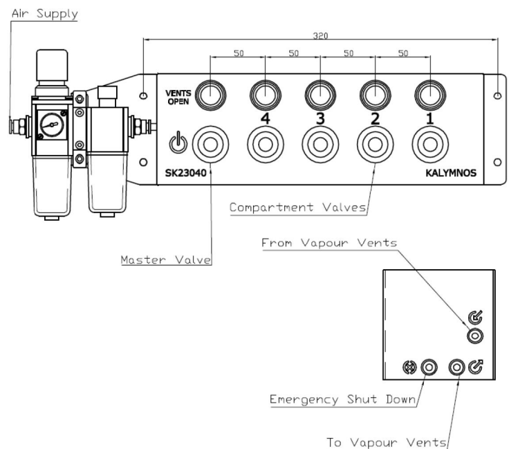
Overall Dimensions – SK23040
