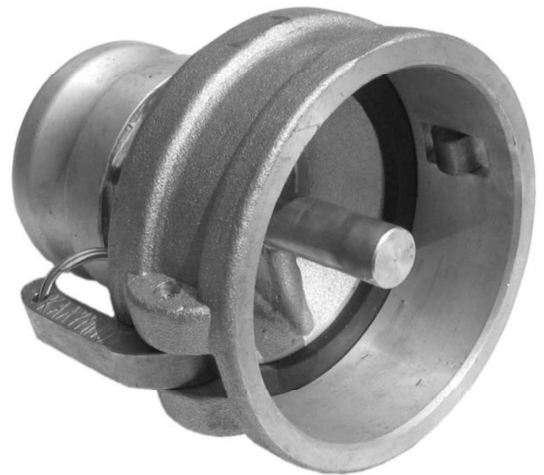
Vapour Recovery Coupler w male 3" adaptor
